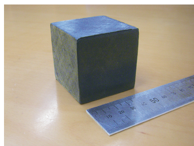
Photo 1) 5cm cubic rubber to be put into the tumbling machine
